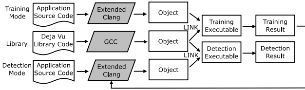
Figure 4: Workflow of DÉJÀ VU.
