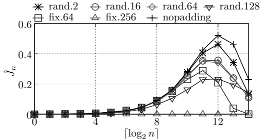
(b) \hat{J}_n for different n
