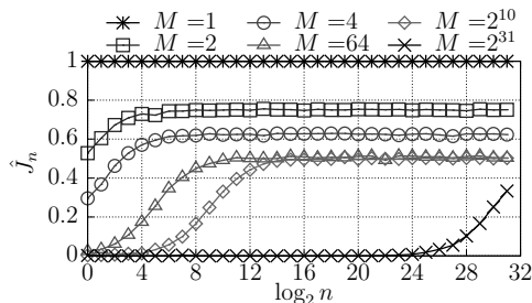
(b) \hat{J}_n for different n and M
