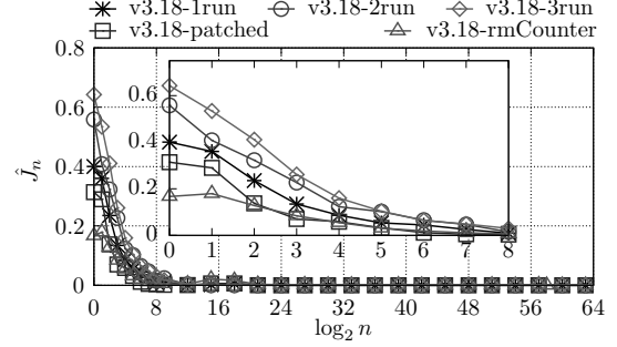
(a) \hat{J}_n per n and version of tcp_rcv_established
