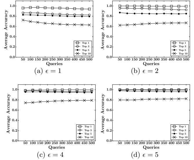
Figure 6: Average rank accuracy based on %CPU field
