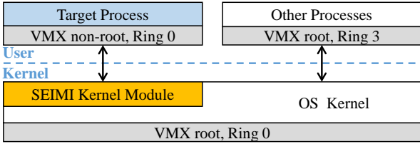
Fig. 2: The architecture overview of SEIMI.
